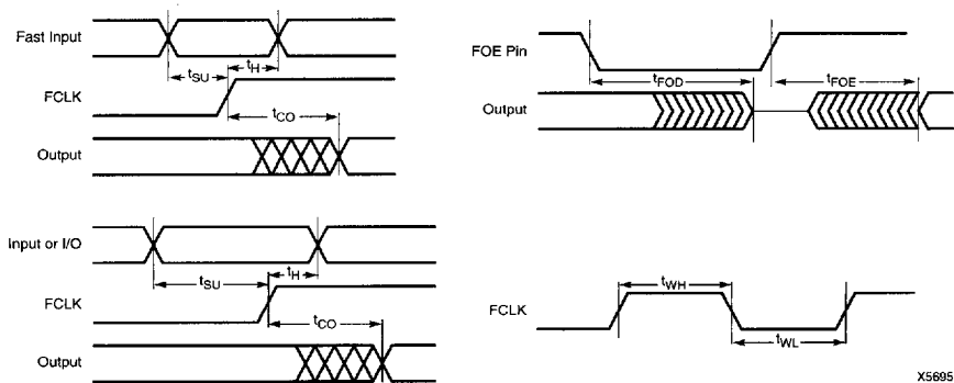
Figure 4: Switching Waveform
