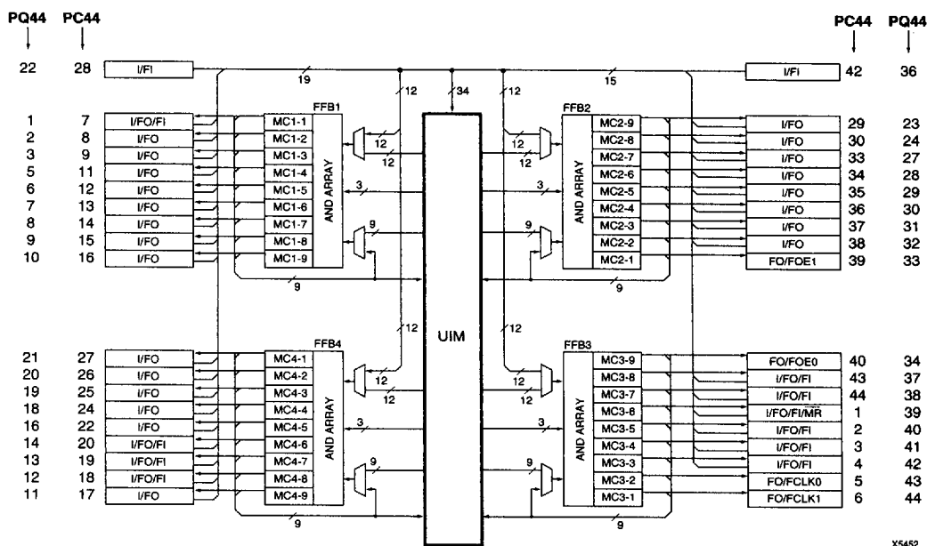
Figure 1: XC7336 Architecture
