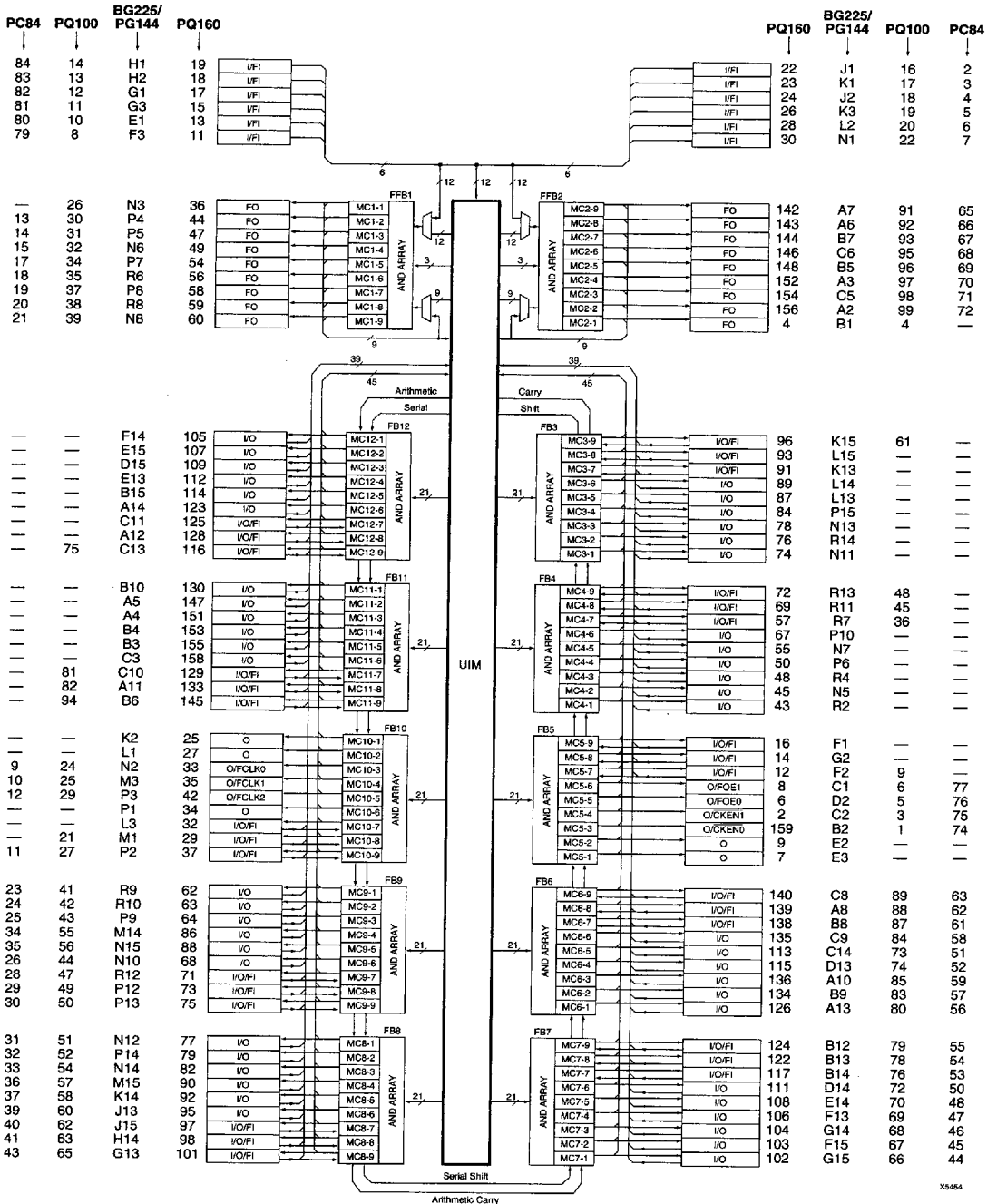
Figure 2: XC73108 Architecture
