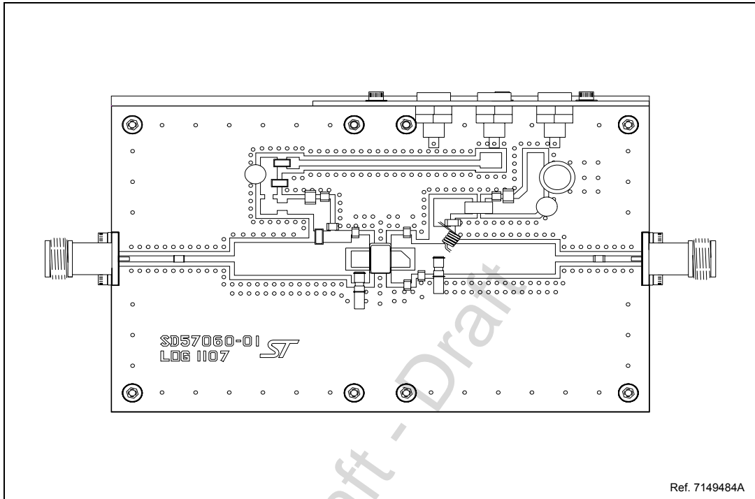
Figure 13. Test fixture
