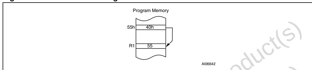
Figure 11. Indirect addressing
