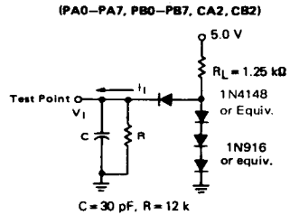
FIGURE 3 — TTL EQUIVALENT TEST LOAD
