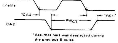
FIGURE 7 -- CA2 DELAY TIME (Read Mode; CRA-5=CRA3=1, CRA-4=0)
