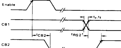
FIGURE 12 -- CB2 DELAY TIME (Write Mode; CRB-5=1, CRB-3=CRB-4=0)
