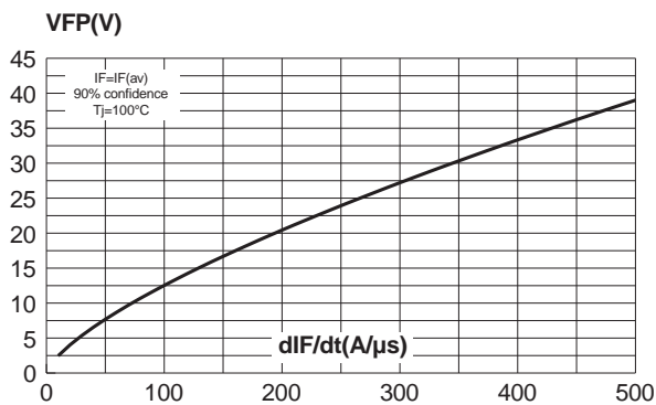
Fig. 10: Transient peak forward voltage versus dl_F/dt (per diode for ISOTOP).
