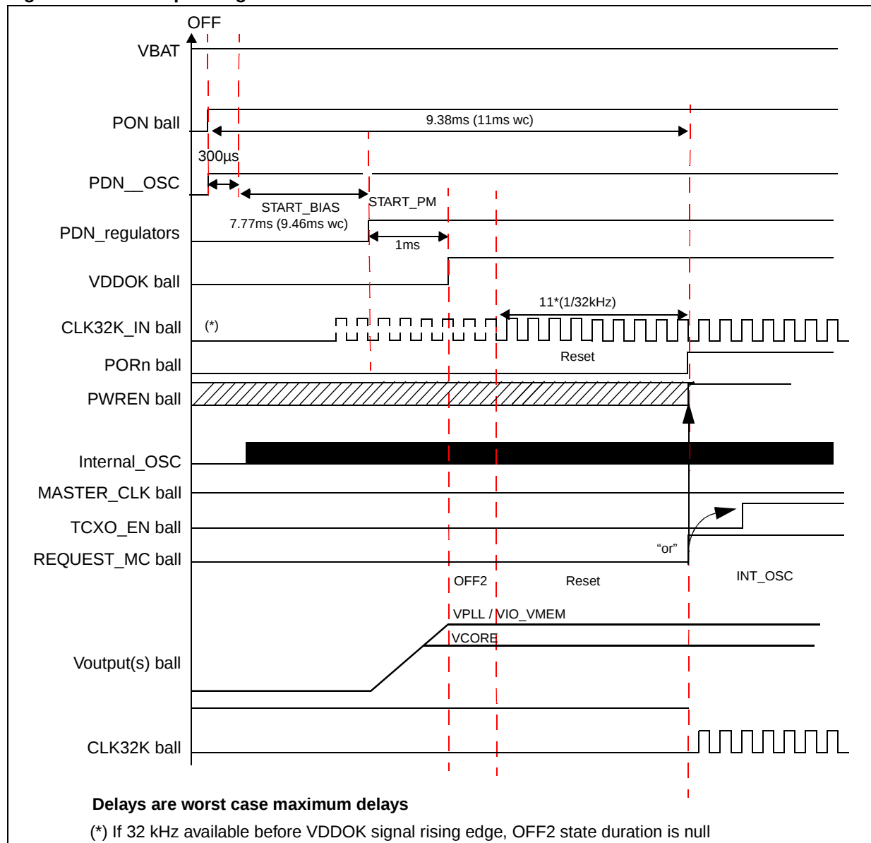
Figure 3. Start-up timing
