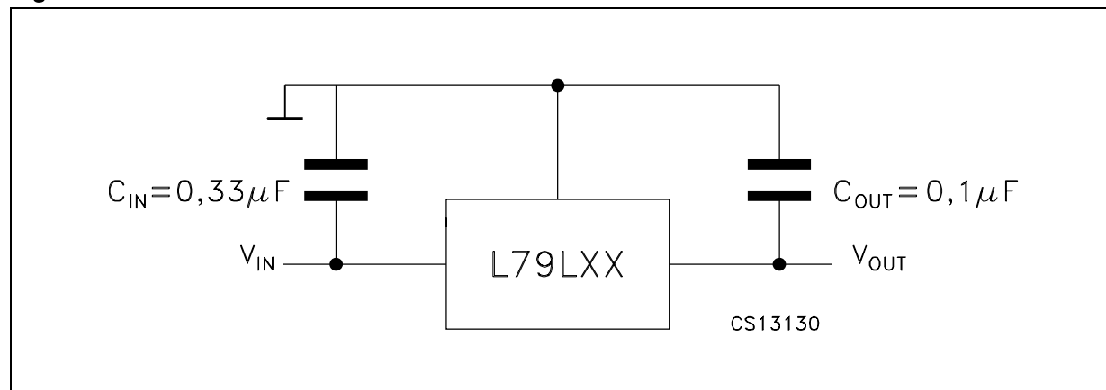
Figure 3. Test circuit
