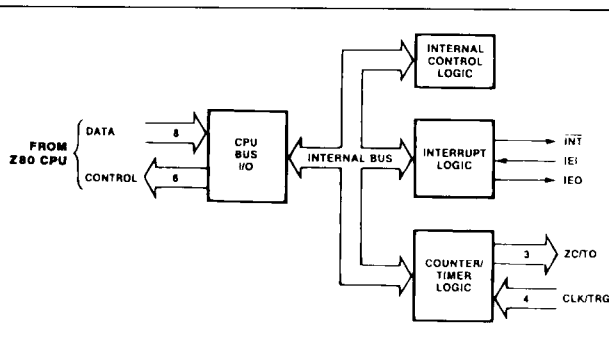
Figure 3 : Functional Block Diagram.
