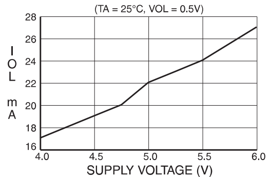
OUTPUT SINK CURRENT vs SUPPLY VOLTAGE
