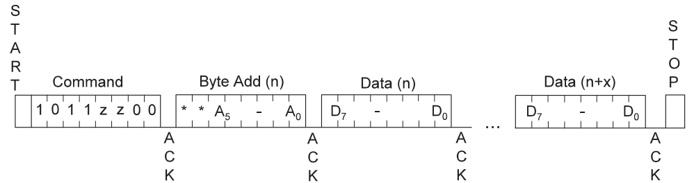
Figure 5. Write EEPROM
