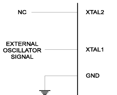
Figure 2. External Clock Drive Configuration
