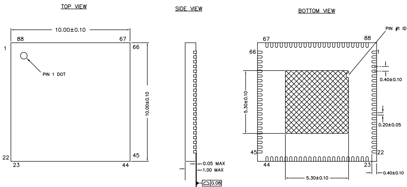
Figure 19. 88-pin QFN ( 10 \times 10 \times 1.0 mm) LT88B 5.3 \times 5.3 EPAD (Sawn) Package Outline
