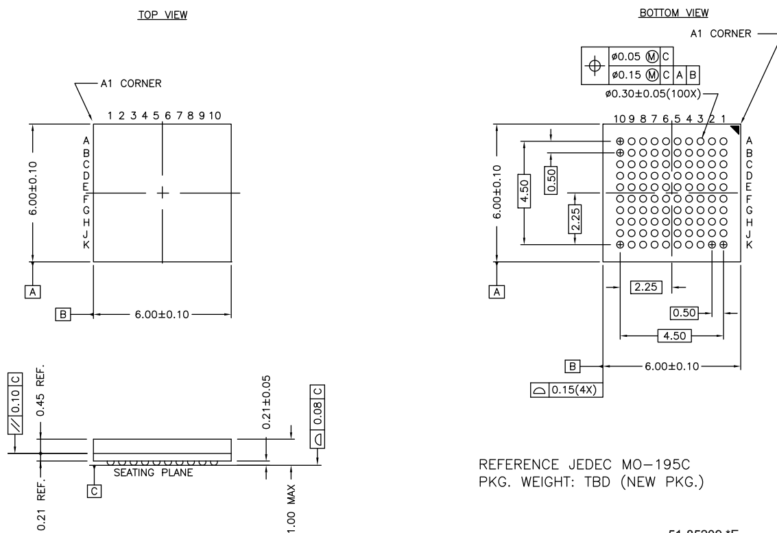
Figure 20. 100-Ball BGA (6.0 × 6.0 × 1.0 mm) BZ100 Package Outline
