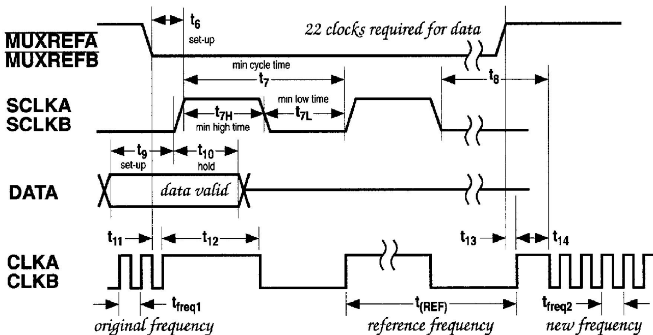
Fig. 4: Serial Programming Timing
