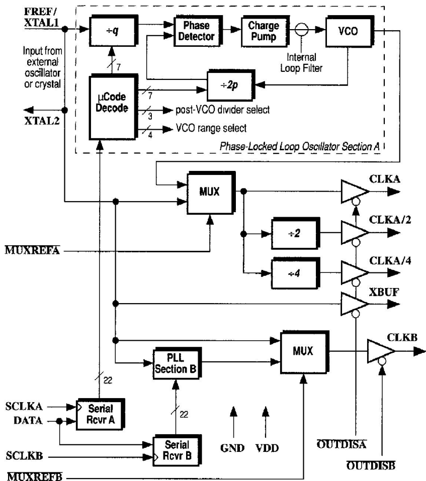
Fig. 1: ICD2051 Block Diagram
