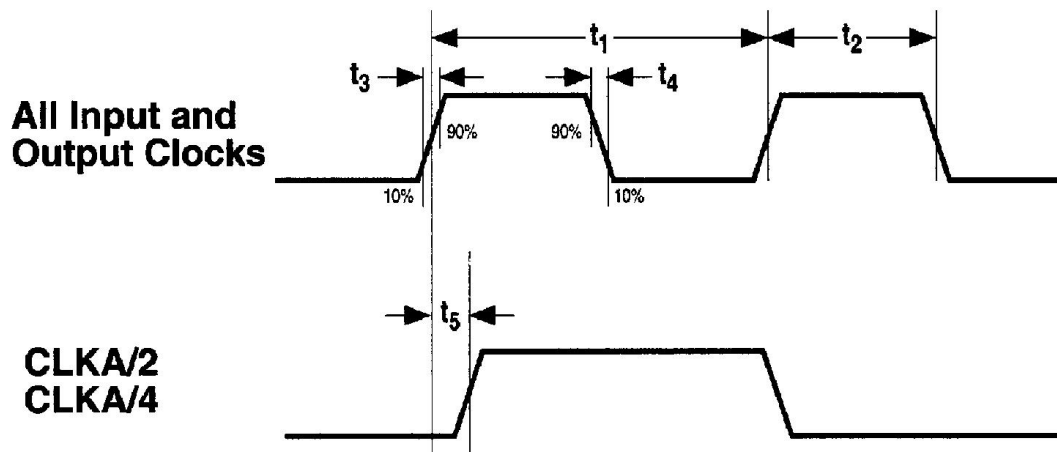
Fig. 3: Rise and Fall Times
