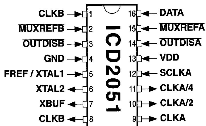
Fig. 2: Pin Descriptions
