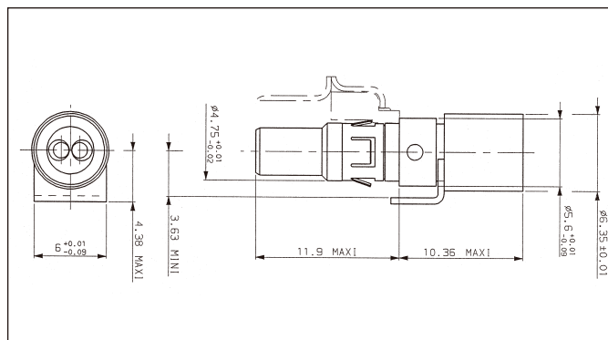
Male straight termination
