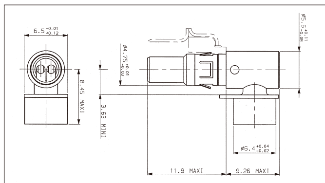
Male 90° termination
