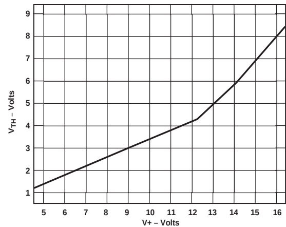
Figure 1. Logic Threshold (AD571K Only)
