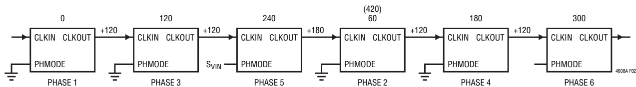
Figure 2. 6-Phase Operation
