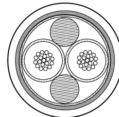
Twisted Pair (Simplex)
